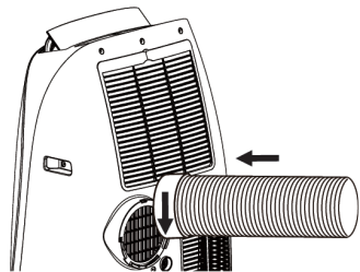
Plastic Hose: Dia. 5.9" (15cm) Length: 14.2" to 47.2" (36cm to 120cm)
