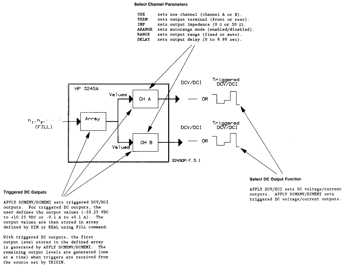
Figure 3-1. DC Outputs - Channel Operation
