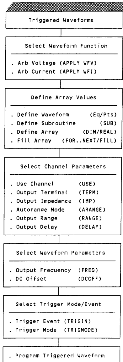
Figure 12-8. Triggered Waveforms - Selection Steps
