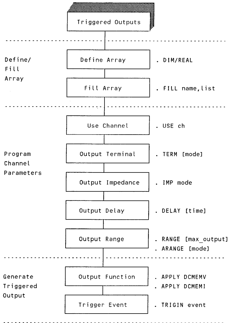
Figure 10-10. Triggered DC Outputs - Programming Sequence
