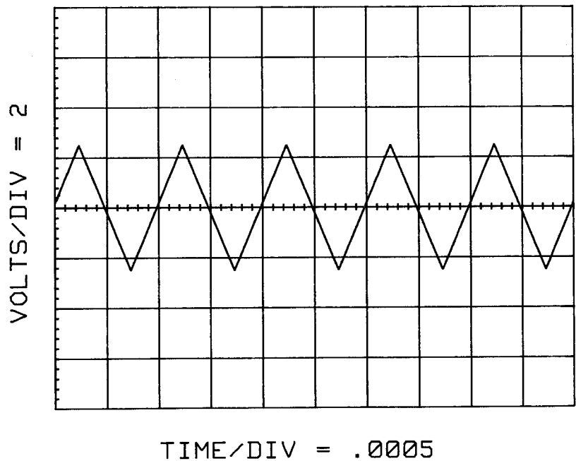
Figure 5-10. Example: Precomputed Ramp Waveform
