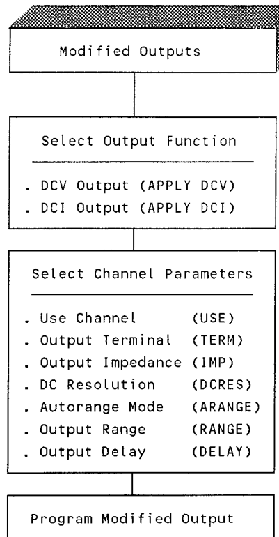
Figure 10-5. Modified DC Outputs - Selection Steps
