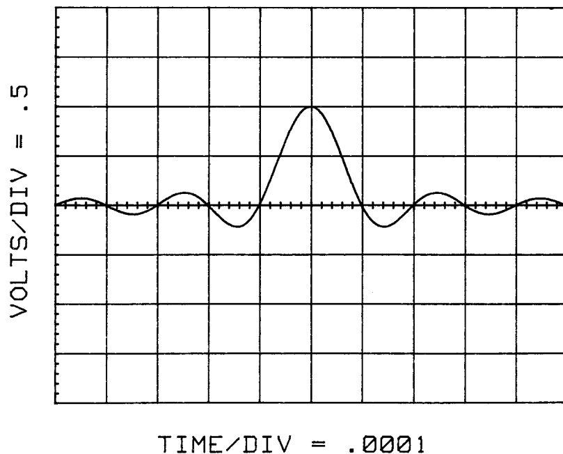
Figure 5-2. Example: Sin(x)/x
