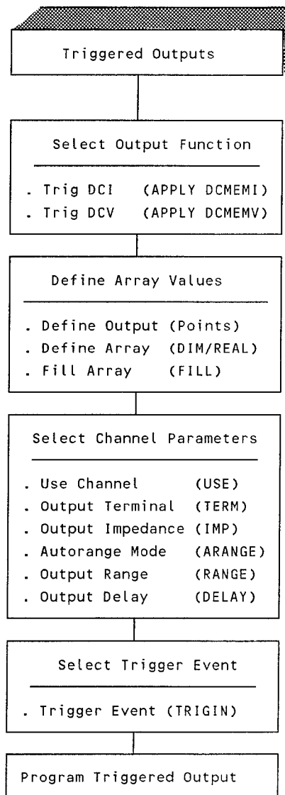
Figure 10-8. Triggered DC Outputs - Selection Steps
