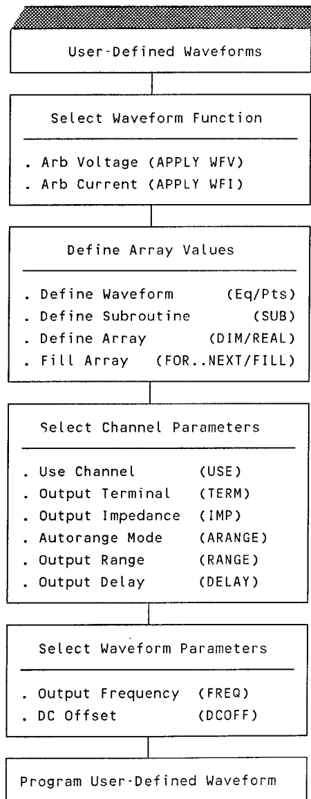
Figure 12-2. User-Defined Waveforms - Selection Steps
