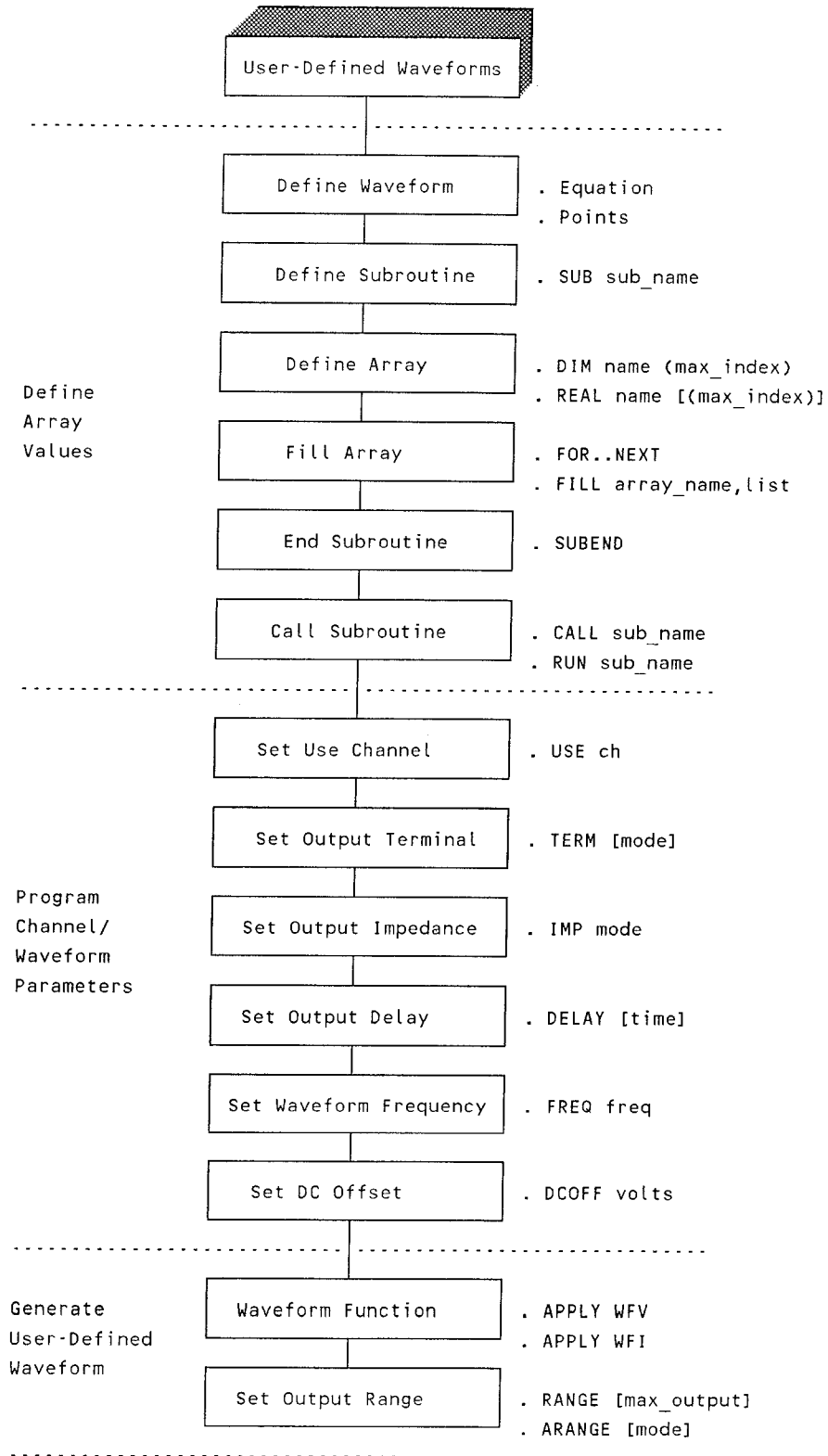
Figure 12-4. User-Defined Waveforms - Programming Sequence
