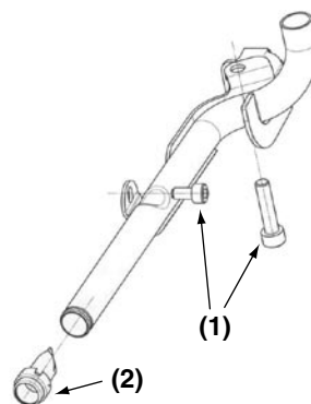
(1) Bolt (2) Spark arrester
