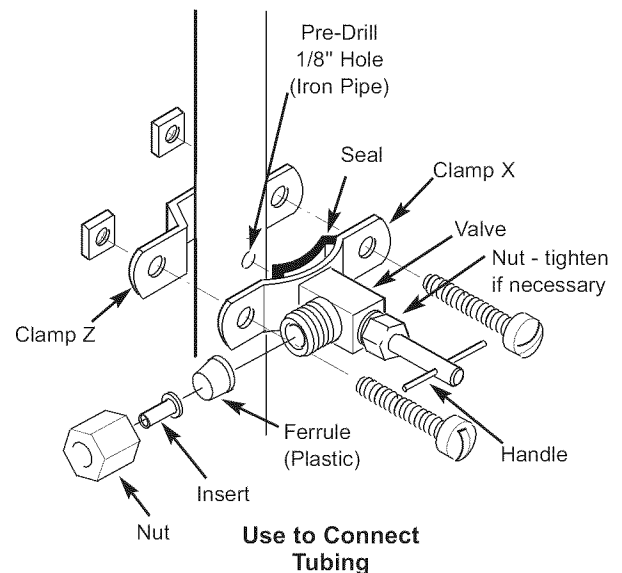
Saddle Valve Connection (Included in package)
