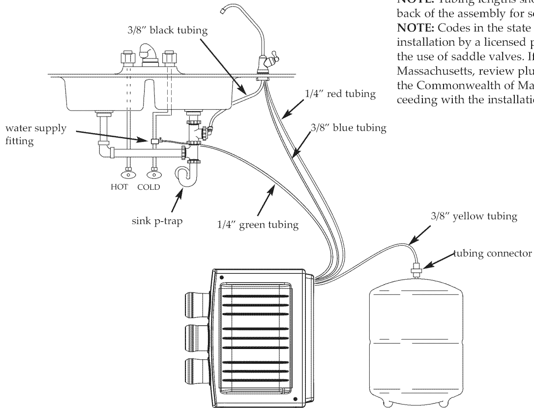
Tube Connections
