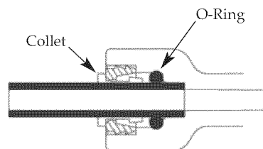
Tube Fully Engaged With Fitting
