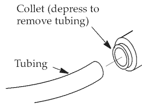
Disconnect Tubing
