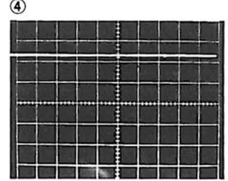
④ 5 mS/cm, .5 V/cm, DC coupled: Confirm Zener diode D1.
