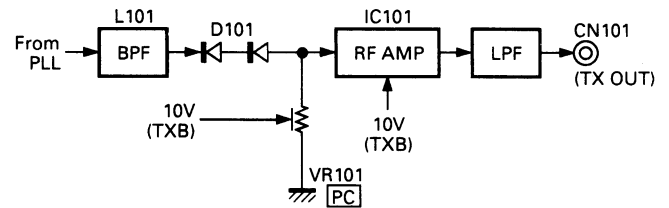
Fig. 7 Drive amplifier
