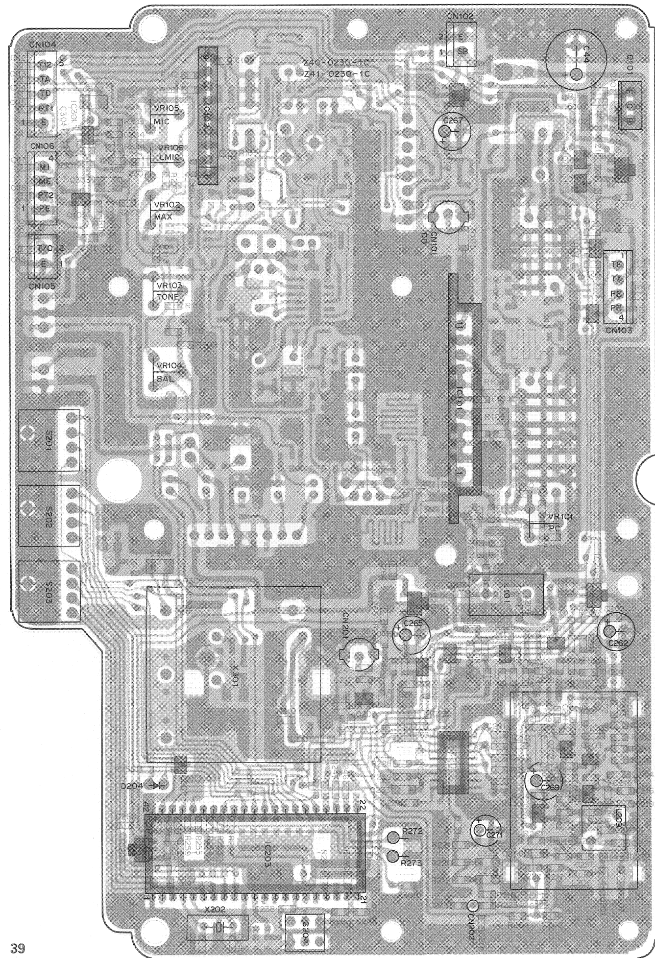
TX UNIT (X56-3020-11) Component side view
