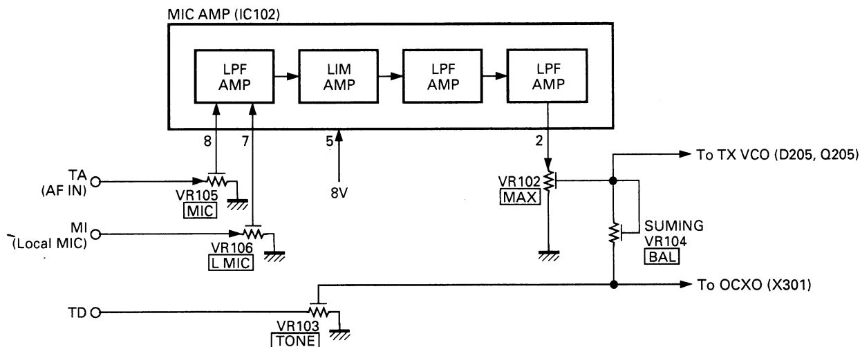
Fig. 5 Microphone amplifier
