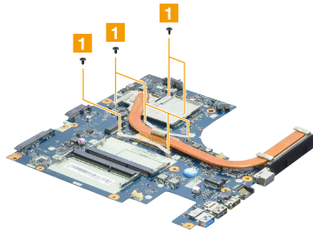
Figure 12. Removal steps of heat sink assembly
