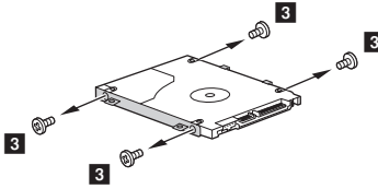
Figure 2. Removal steps of hard disk drive (continued)
