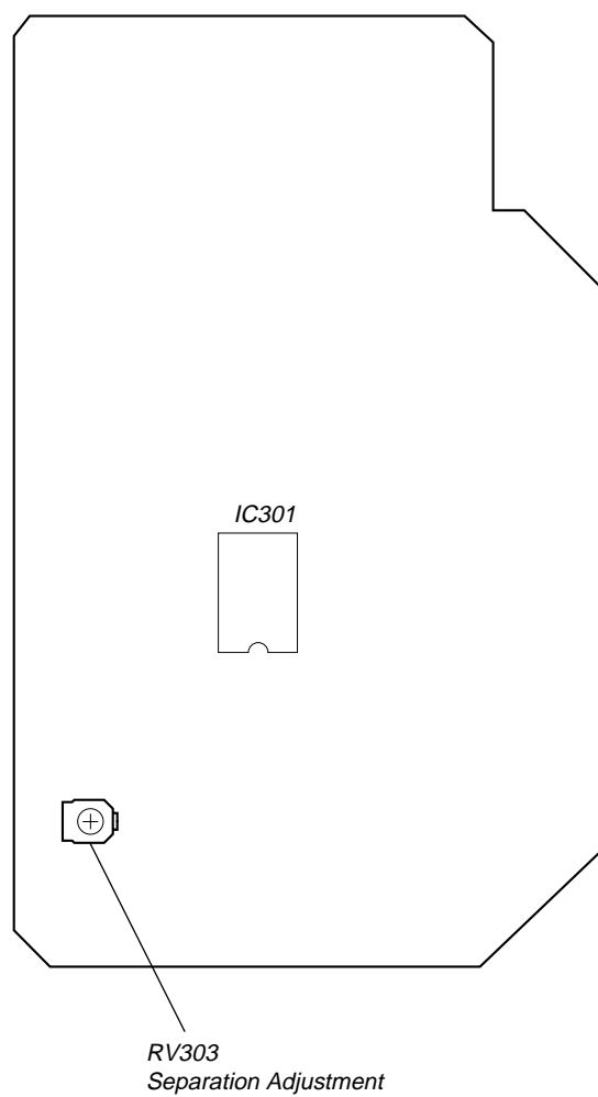
[RX-BASE board] – Conductor Side –
