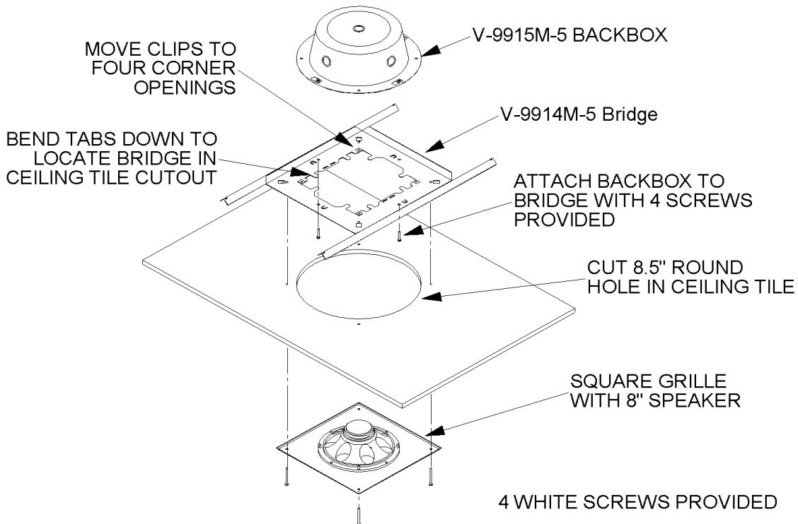
FIGURE 2: CEILING INSTALLATION INSTRUCTIONS
