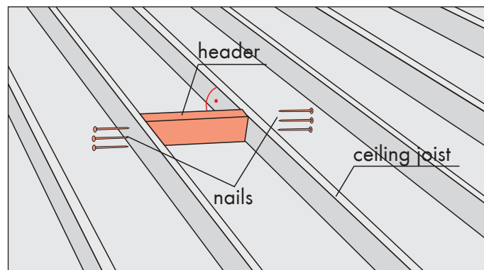
Fig.13. Nail the header at both ends.
