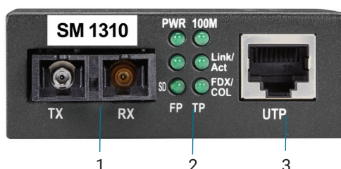
FIGURE 2-5. LHC212A FRONT PANEL
