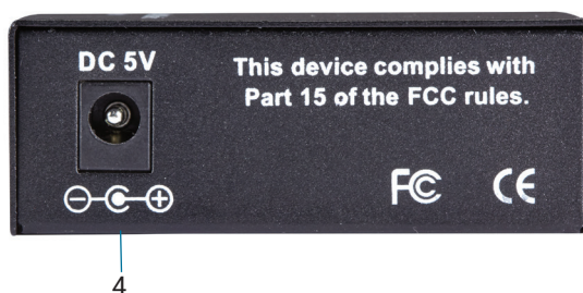
FIGURE 2-8. LGC210A BACK PANEL
