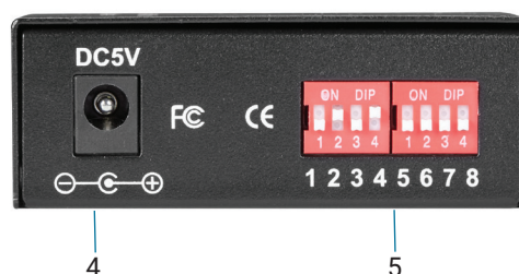
FIGURE 2-6. LHC212A BACK PANEL
