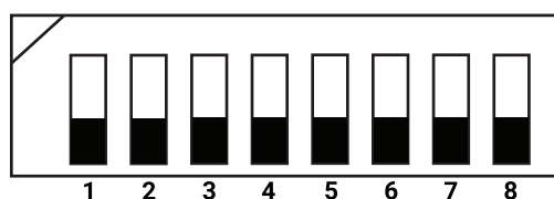
FIGURE 3-1. DIP SWITCH ON THE LHC210A, LHC211A AND LHC212A
