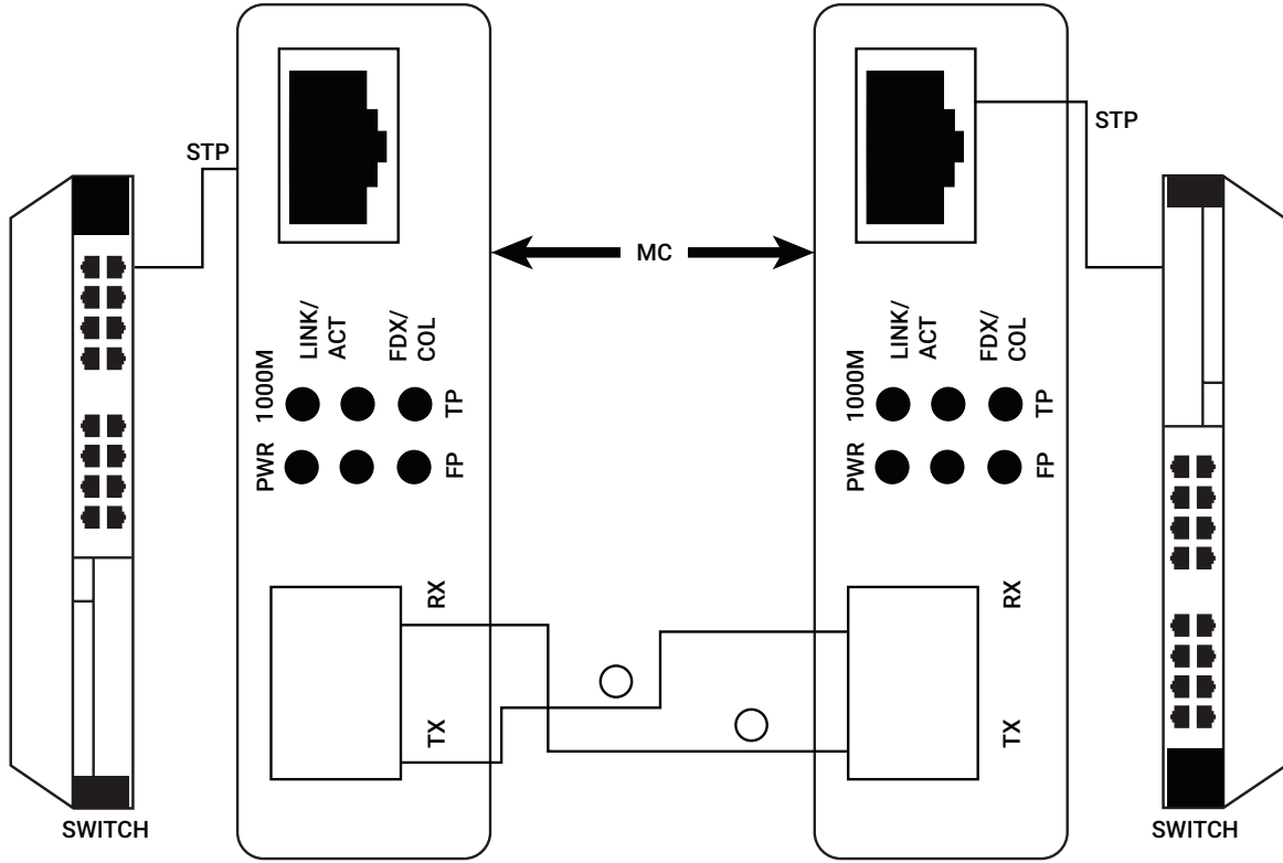
FIGURE 3-2. TYPICAL INSTALLATION
