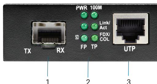
FIGURE 2-1. LHC210A FRONT PANEL
