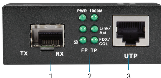
FIGURE 2-7. LGC210A FRONT PANEL
