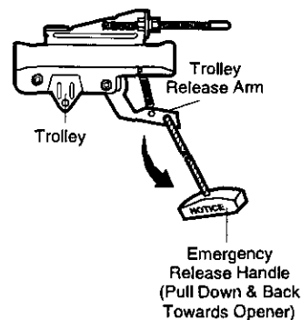
Lockout position
