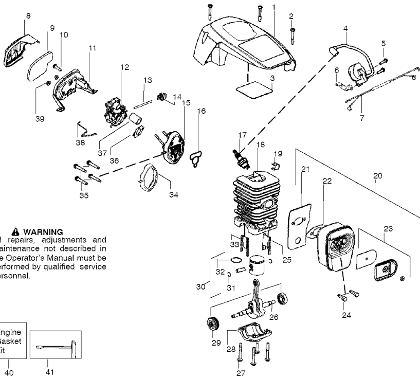
SEARS CHAINSAW MODEL 358.351800
