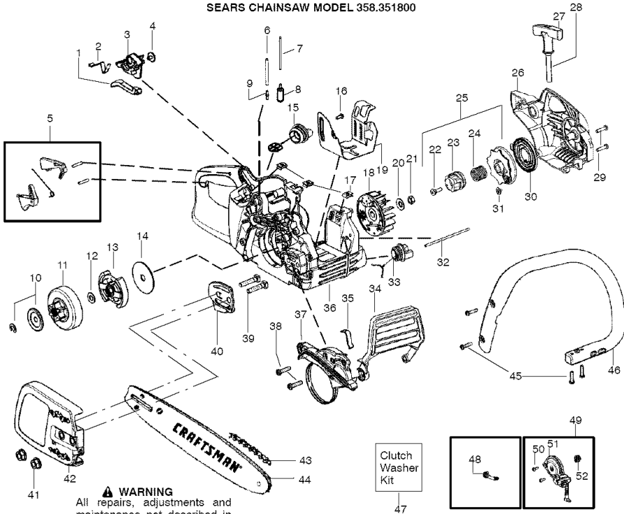
SEARS CHAINSAW MODEL 358.351800
