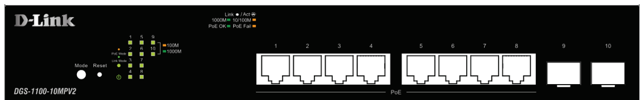
Figure 2-7 – DGS-1100-10MPV2 Front Panel
