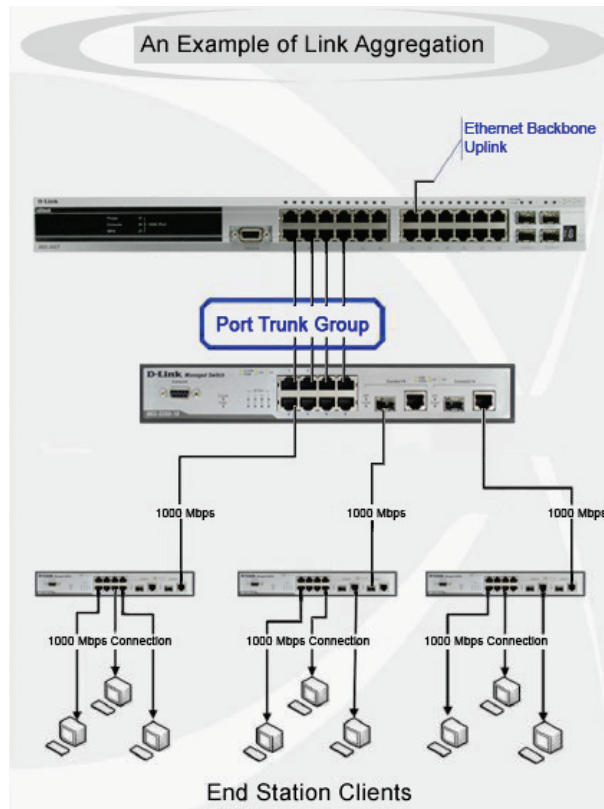
Figure 7-29 Example of Port Trunk Group
