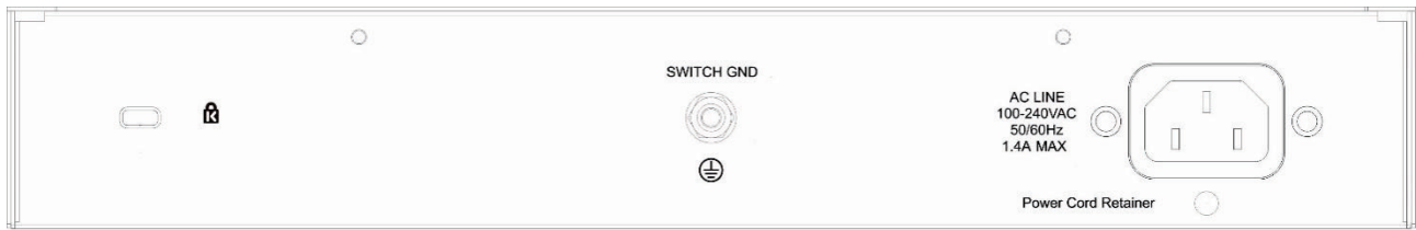
Figure 2-6– DGS-1100-24PV2 Rear Panel
