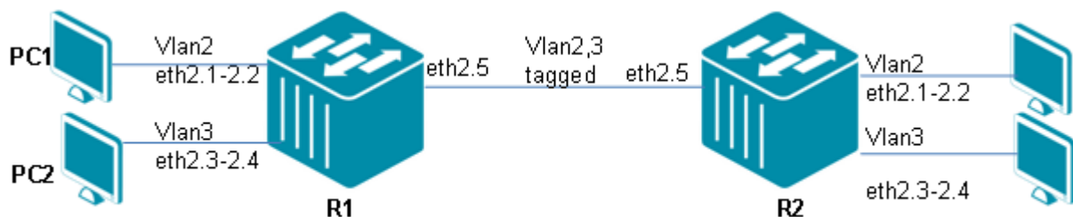
Figure 10-1 Configuration Topology
