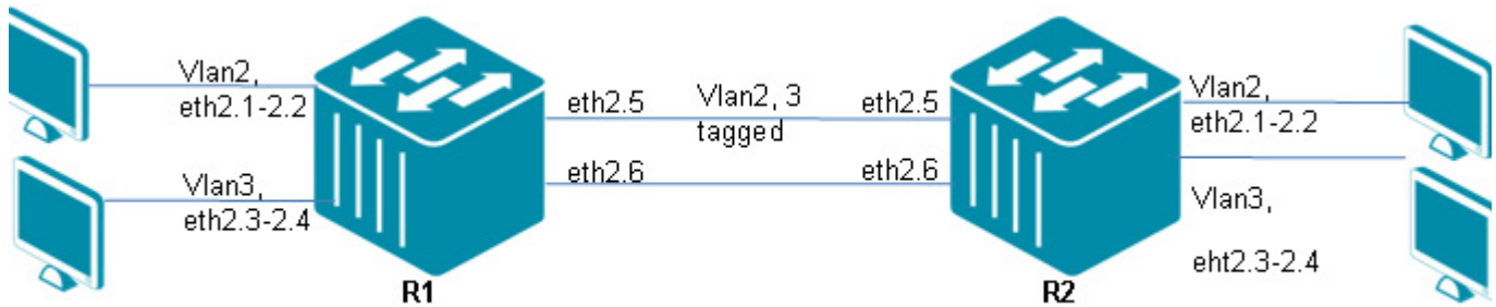
Figure 14-4 MSTP Configuration Topology
