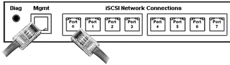
Rear Connection Panel (8-port configuration shown)
