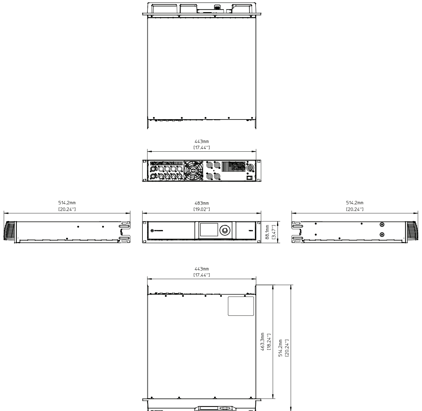
Figure 8.2: Dimensions: TGX
