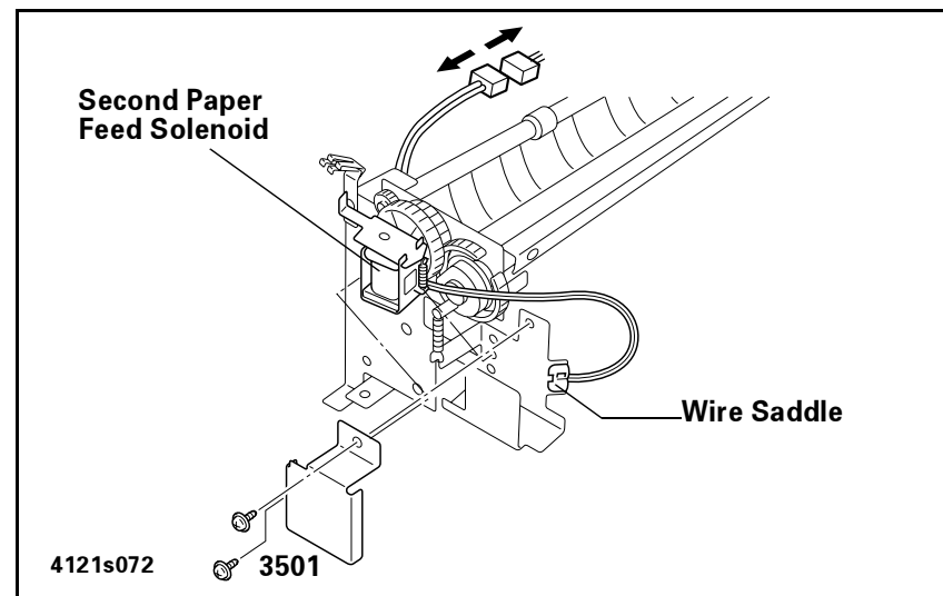
Figure 4-35. Second Paper Feed Solenoid (SL21) Removal
