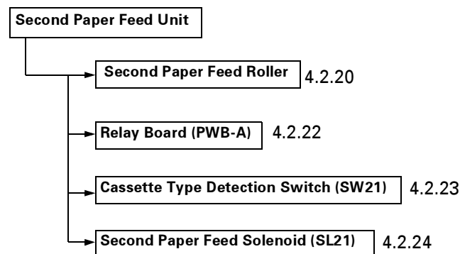
Figure 4-3. Disassembly Flowchart 2
