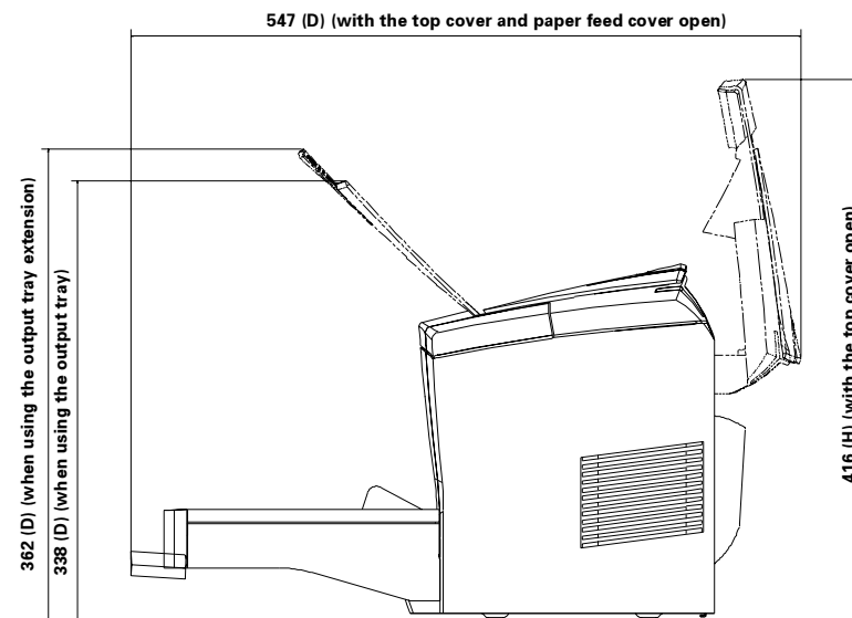
Figure 1-4. Right View
