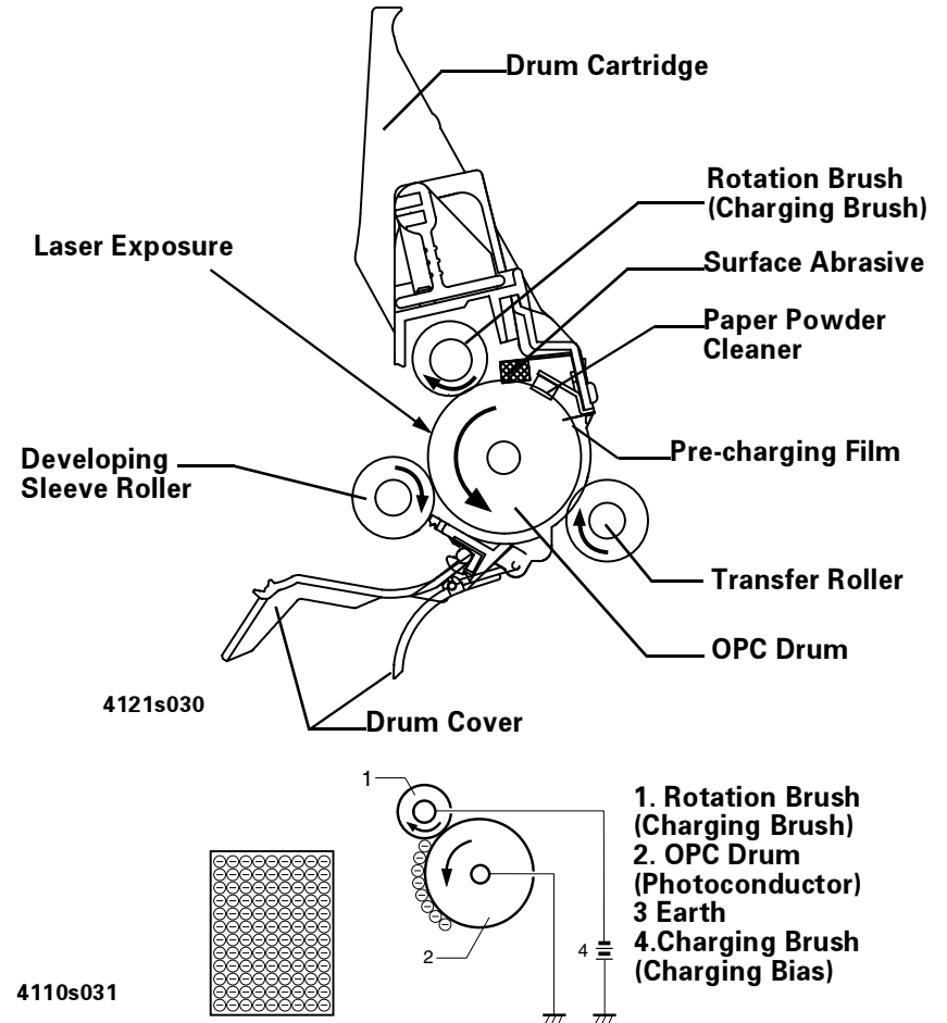
Figure 2-5. Charging Mechanism
