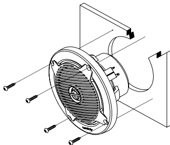
Figure 1. Mounting the Kappa 62m and Kappa 692m.
