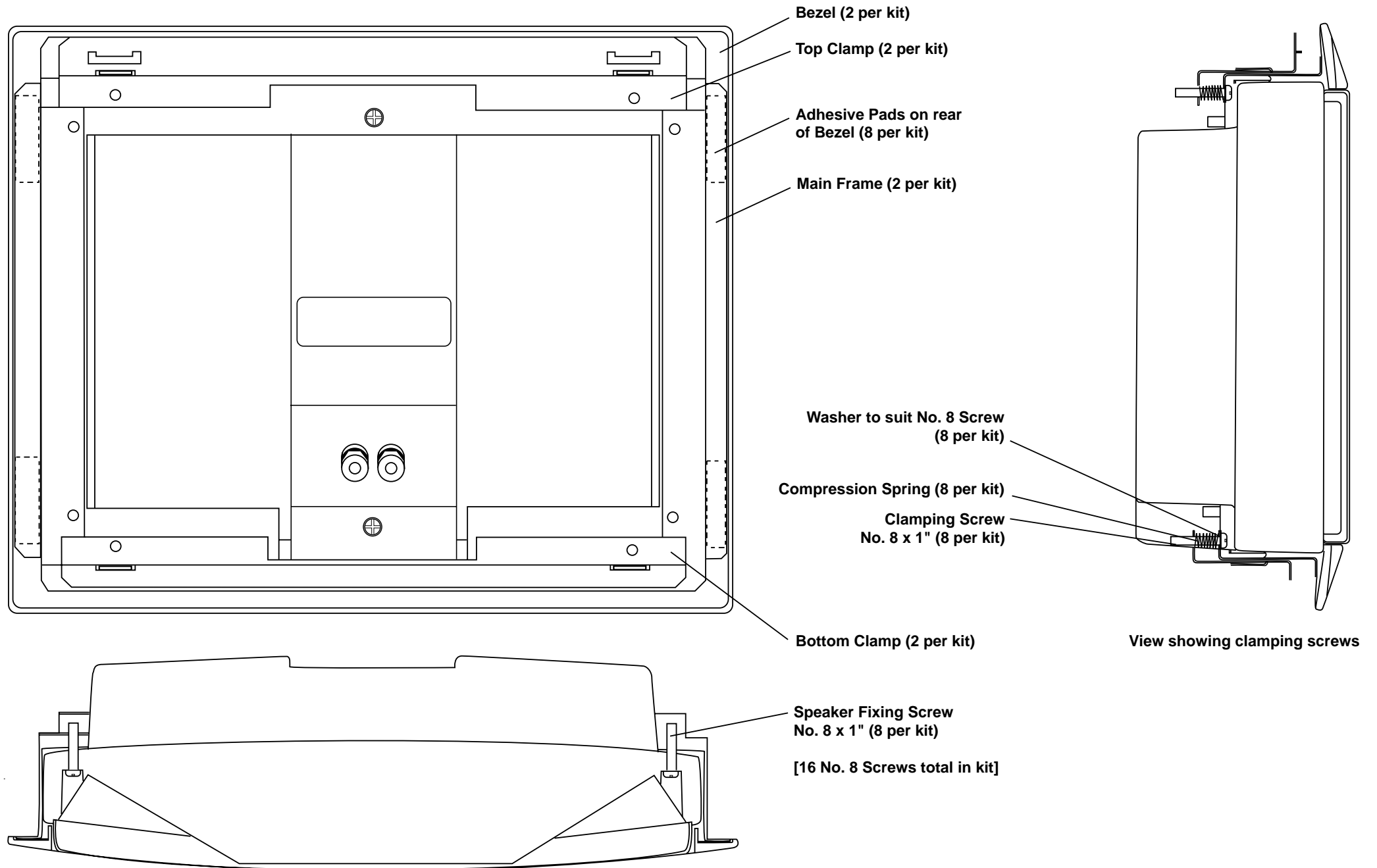
View showing rear of speaker with flush-mount kit in position
