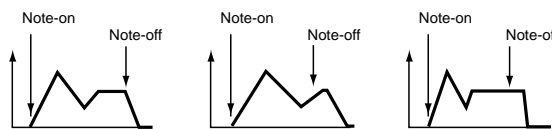
Amp 1 EG changes (Time) (AMS=Velocity, Intensity= a positive (+) value)
