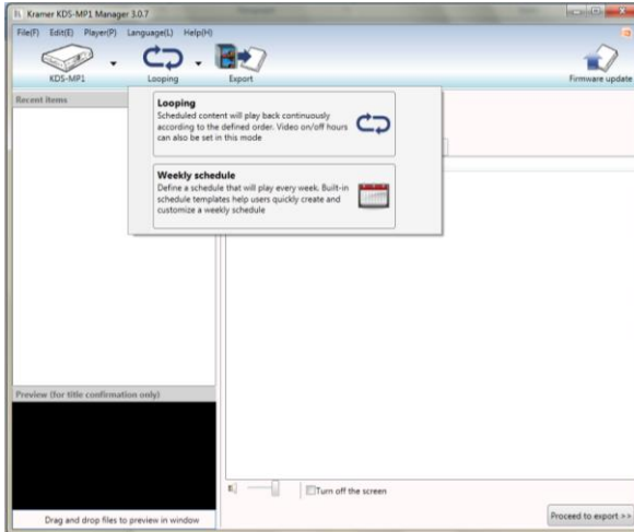
Figure 7: Selecting the Schedule Mode
