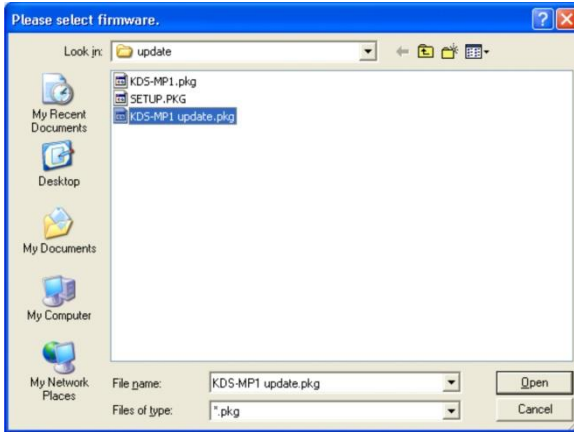
Figure 28: Select Firmware
