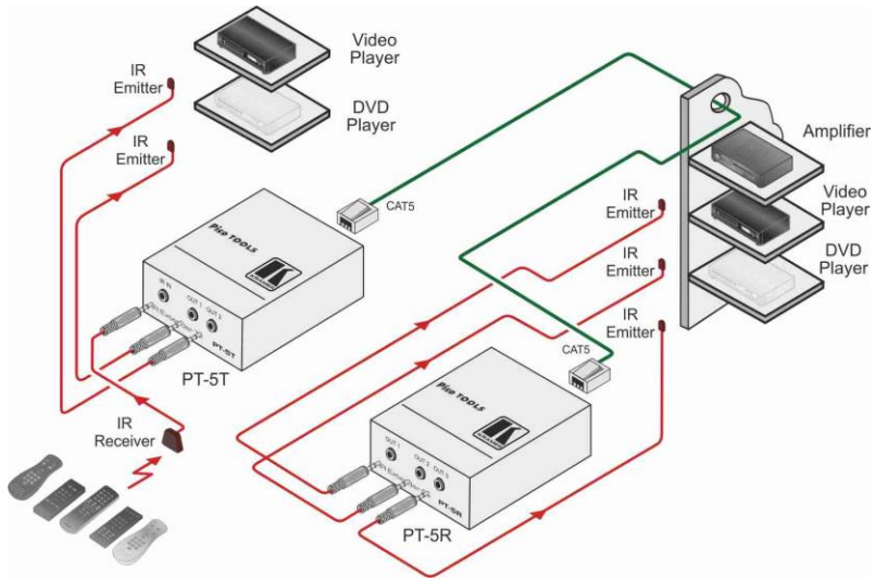
Figure 4: Connecting the PT-5T/R
