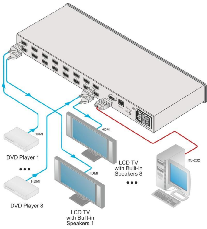
Figure 3: Connecting the VS-88HN 8x8 HDMI Matrix Switcher
