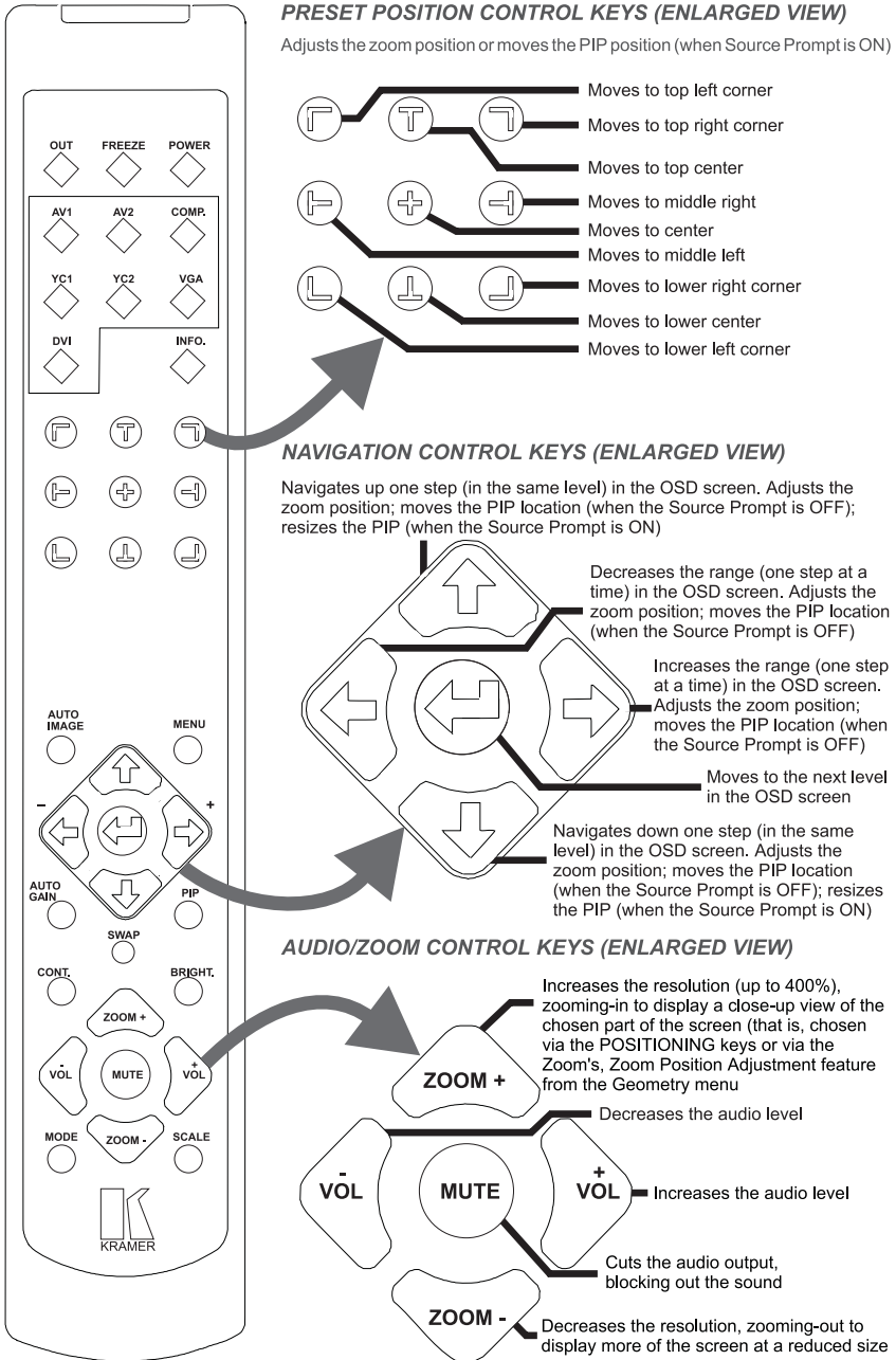
Figure 49: Infra-red Remote Control Transmitter
