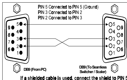
Figure 2: Connecting the PC
