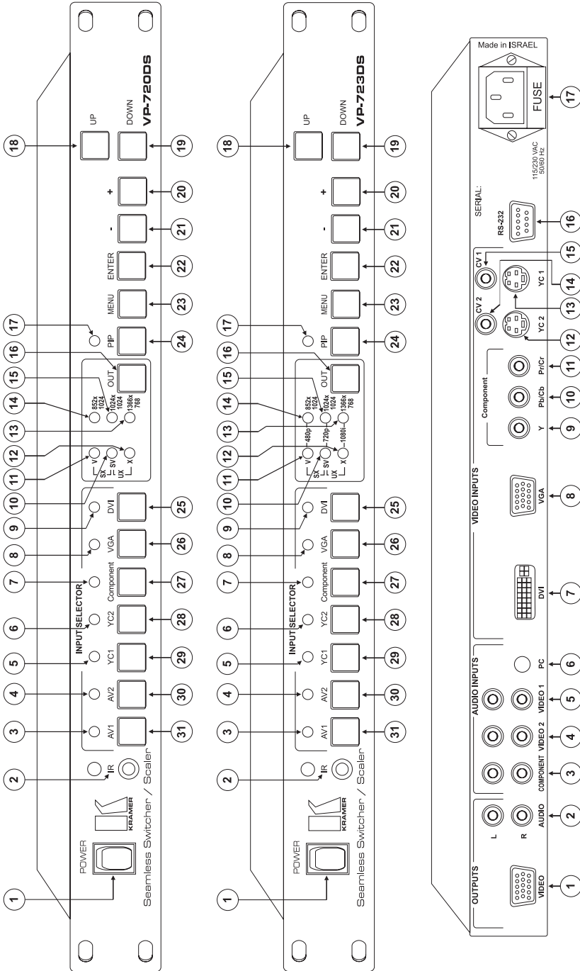
Figure 1: Front Panels of the VP-720DS and VP-723DS, and their Rear Panel
