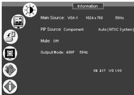
Figure 48: Information Screen
