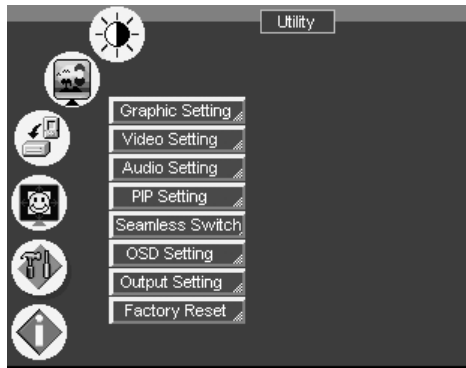
Figure 27: Utility Screen
