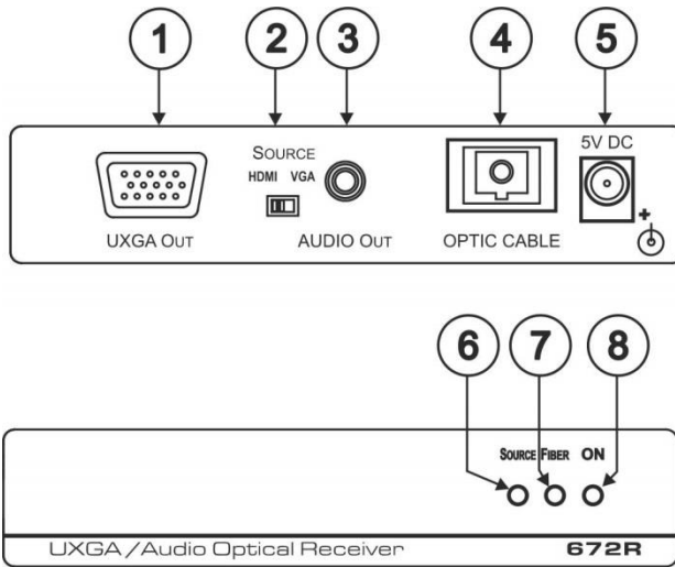
Figure 2: 672R DVI Optical Receiver
