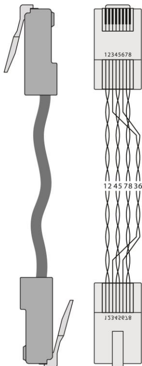
Figure 4: TP PINOUT
