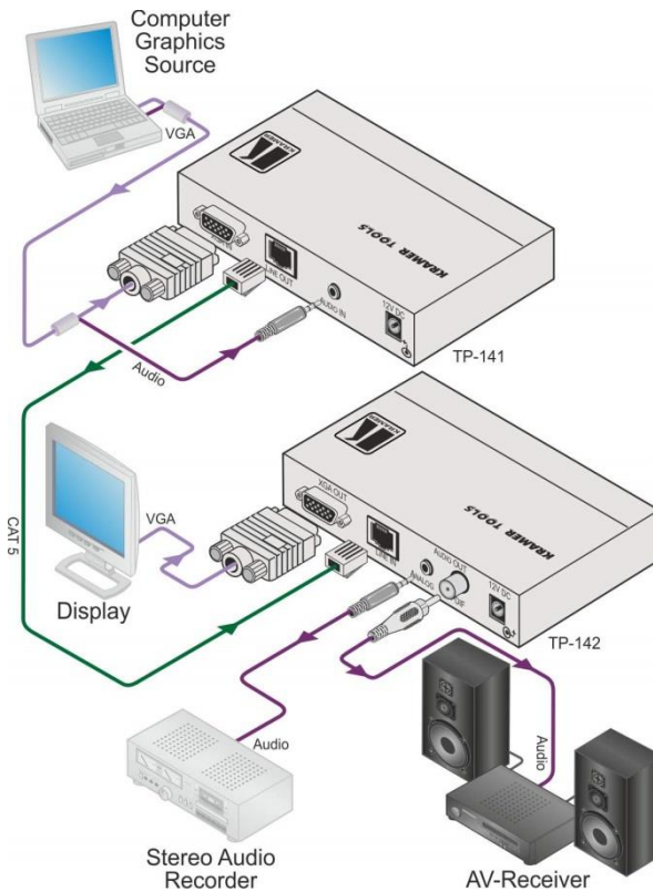
Figure 3: Connecting the TP-141, TP-142
