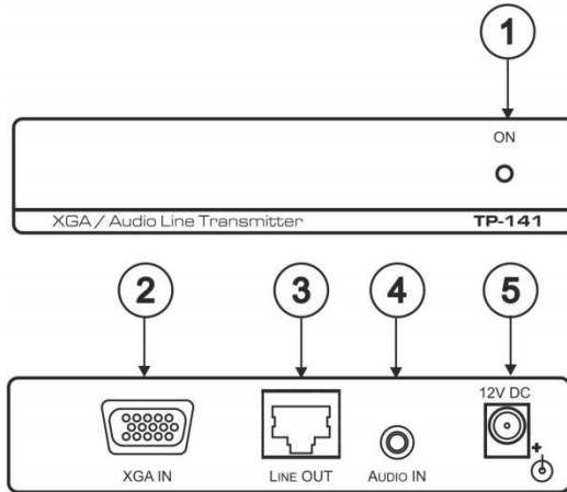
Figure 1: TP-141 XGA/Audio Line Transmitter
