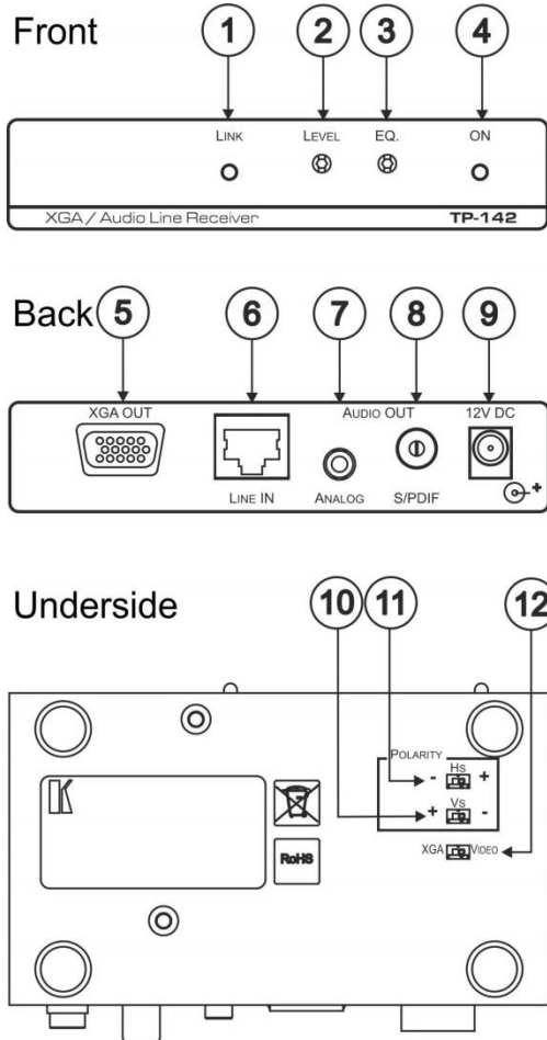
Figure 2: TP-142 XGA/Audio Line Receiver
