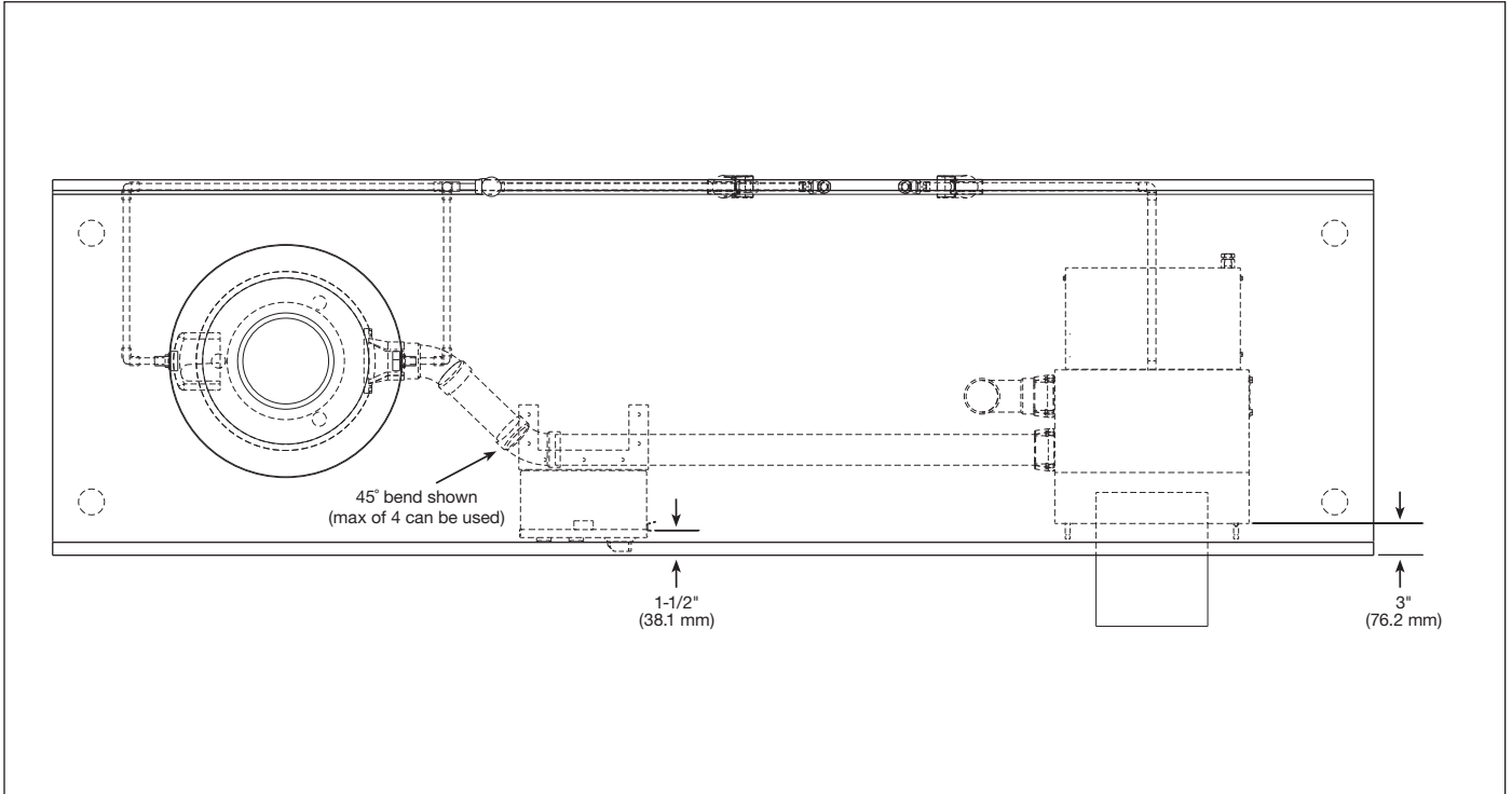
Figure 11. Top View
