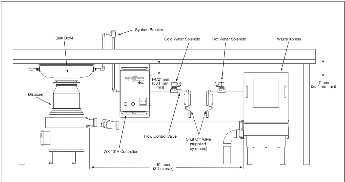
Figure 1. Typical Installation
