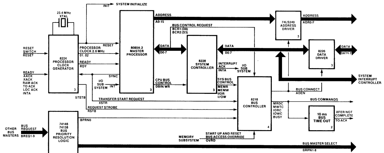
Figure 2-1. IPB Simplified Block Diagram
