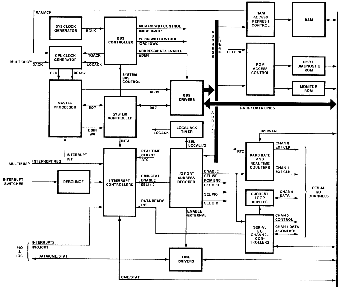
Figure 2-1. IPB Simplified Block Diagram
