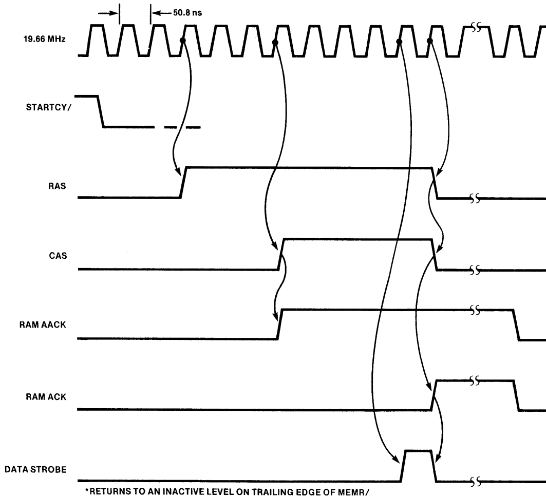
Figure 2-7. RAM Read Cycle Timing
