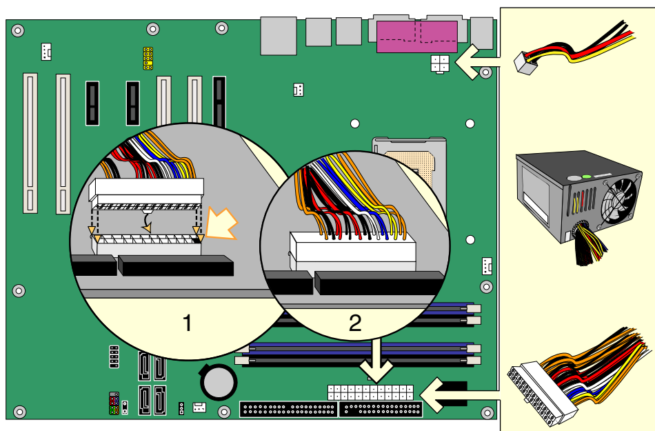
Figure 24. Connecting 2x12 Power Supply Cables
