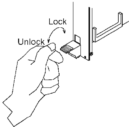
Figure 2.4: Chassis Installation/Removal
