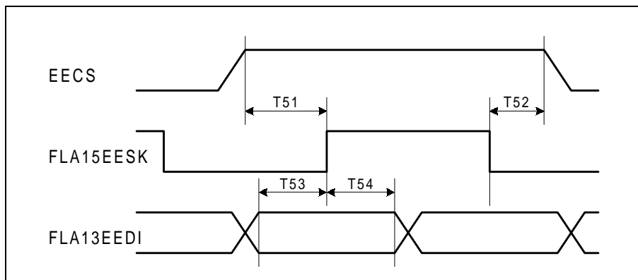
Figure 30. EEPROM Timings
