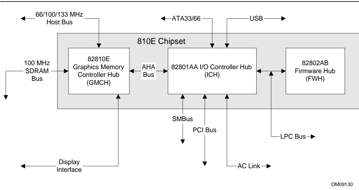
Figure 3. Intel 810E Chipset Block Diagram
