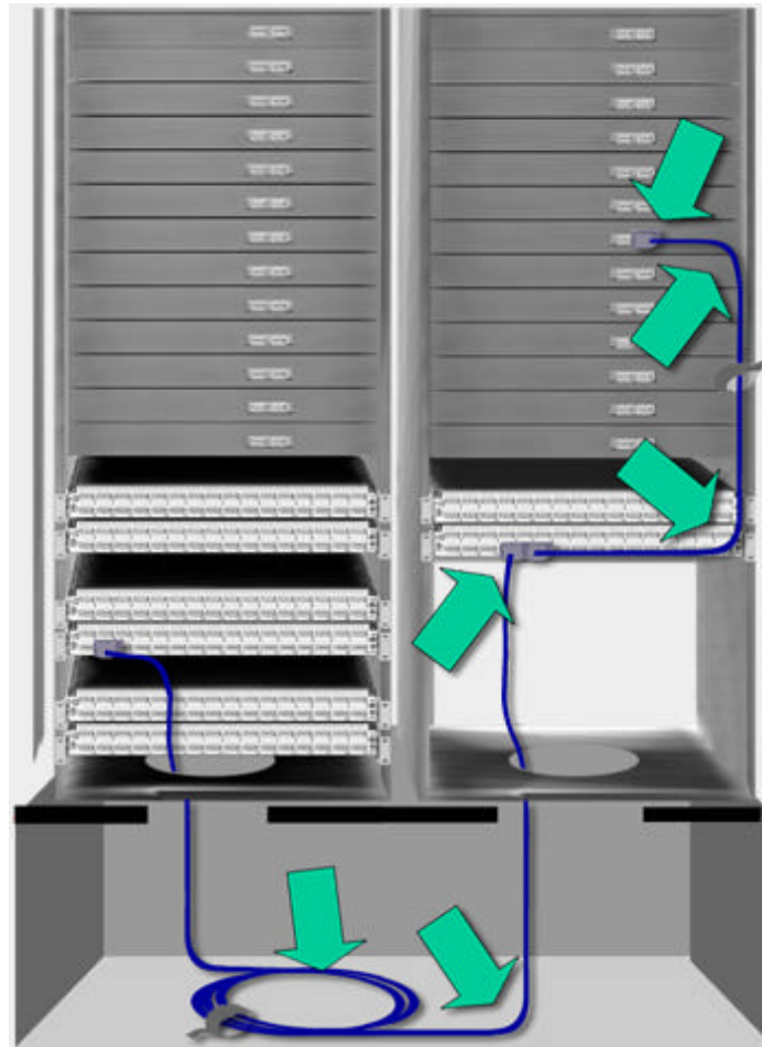
Figure 3. InfiniBand* Cable Bend Radius
