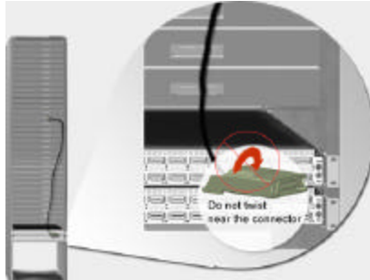
Figure 2. Rotating InfiniBand* Connectors
