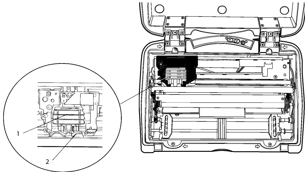
1 Print head 2 Mask spring
