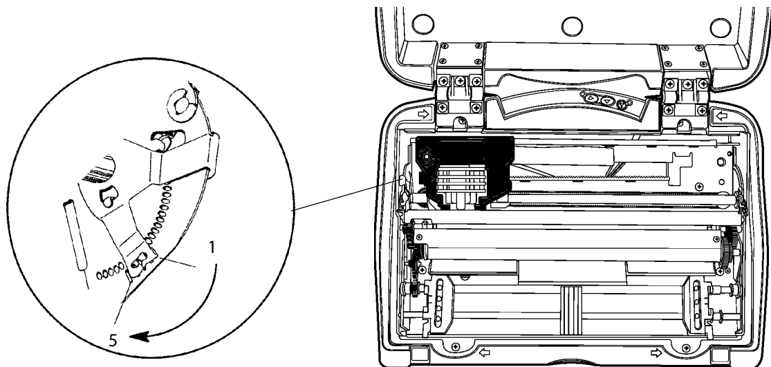
This illustrating shows the print head adjuster set on its third notch.
