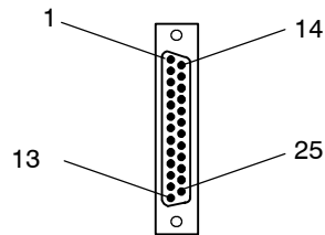
25-Pin DSUB Male
