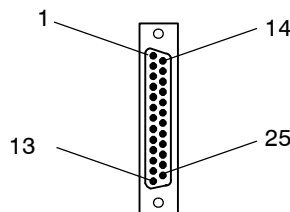
25-Pin DSUB Female
