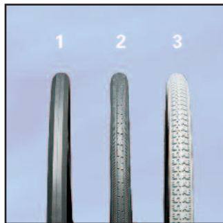
Tires 1. Urethane 2. Urethane - High Profile 3. Pneumatic - Flat-Free All tires available in 20", 22" and 24" sizes. Available on all chairs.
