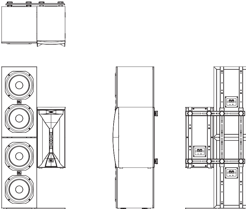
Configuration 4: One SAM1HF and two SAM2LF vertical
