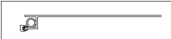
Side profile showing placement of door labyrinth grommet
