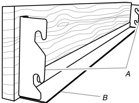
A. Panel brackets B. Grill trim piece
