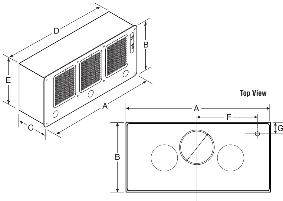
JXT7142 liner for 42" installation
