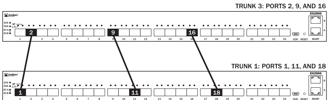
Figure 10: Port Trunk Group Configuration Example
