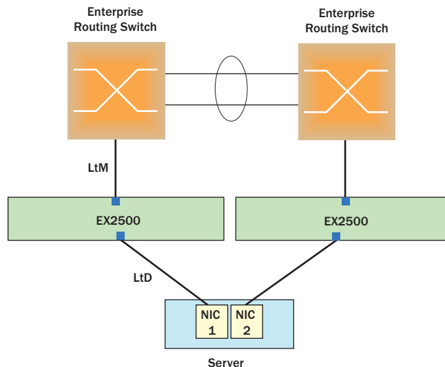
Figure 14: Uplink Failure Detection Example
