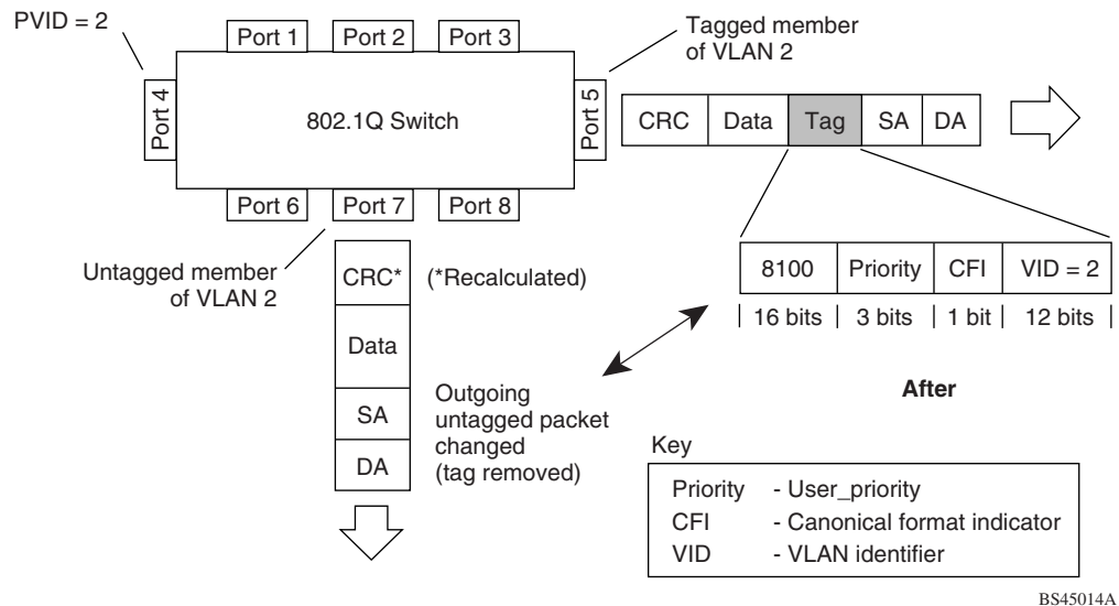
Figure 5: 802.1Q Tagging (after 802.1Q Tag Assignment)
