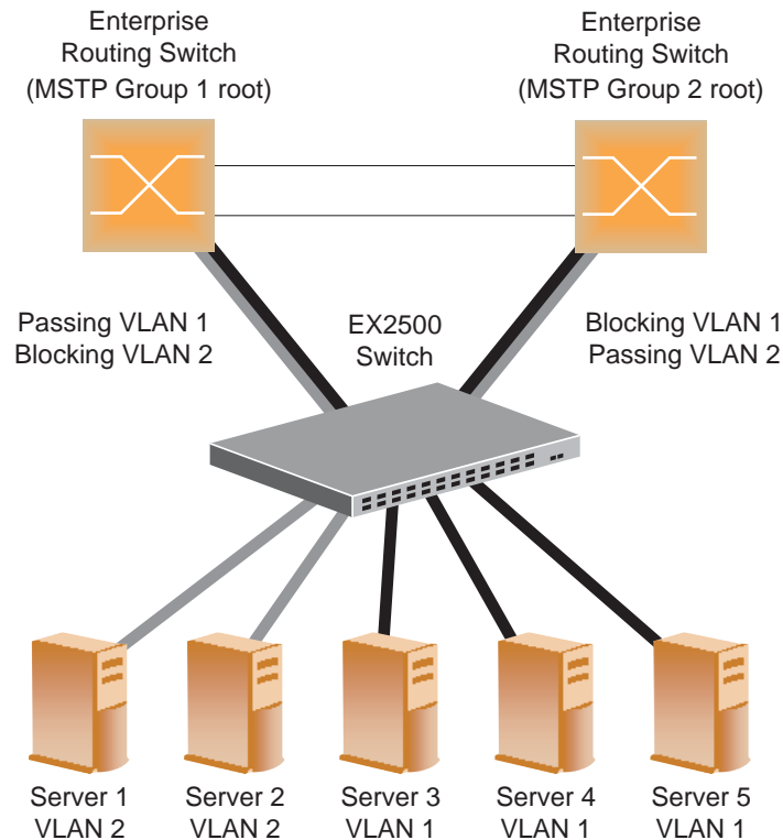
Figure 9: Implementing Multiple Spanning Tree Groups
