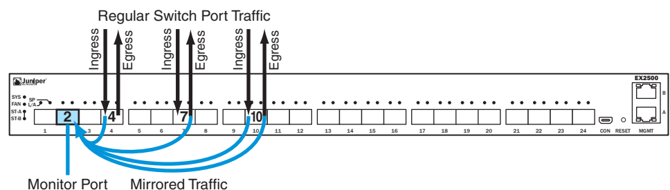
Figure 15: Monitoring Ports
