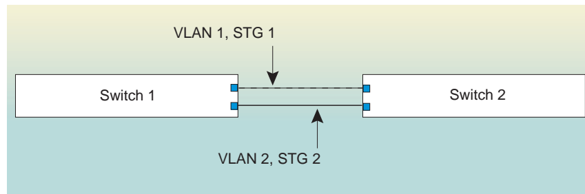
Figure 8: Two VLANs, Each on a Different Spanning Tree Group
