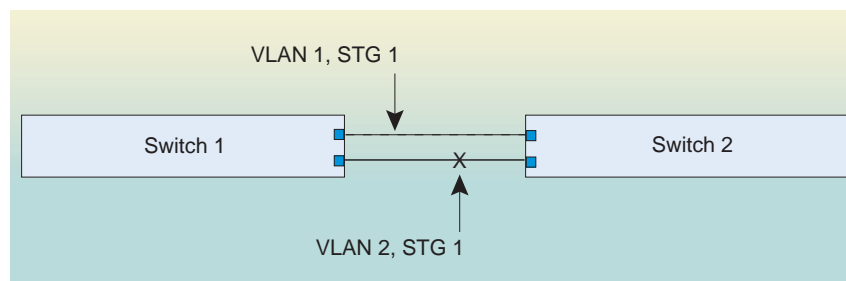
Figure 7: Two VLANs on One Spanning Tree Group
