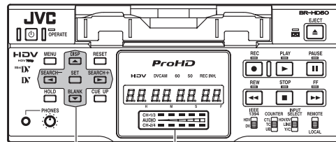
Adjustment buttons
