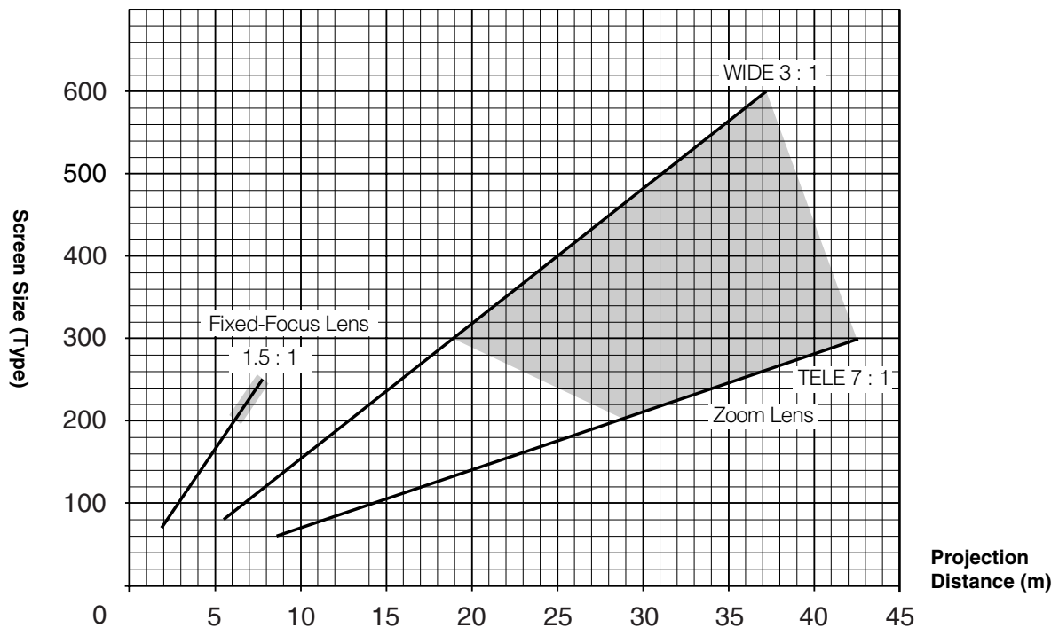
Relationship of screen size vs. projection distance
