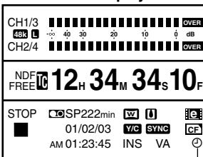
Timer symbol
