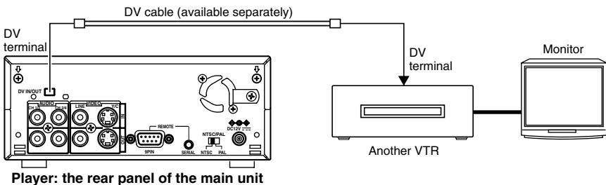
Player: the rear panel of the main unit
