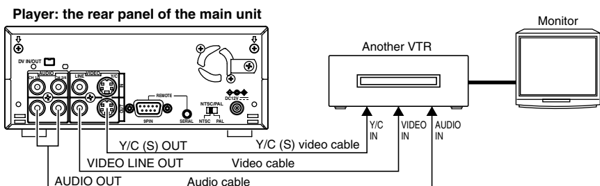
Player: the rear panel of the main unit
