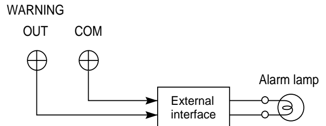
[WARNING OUT] warning signal output terminal
